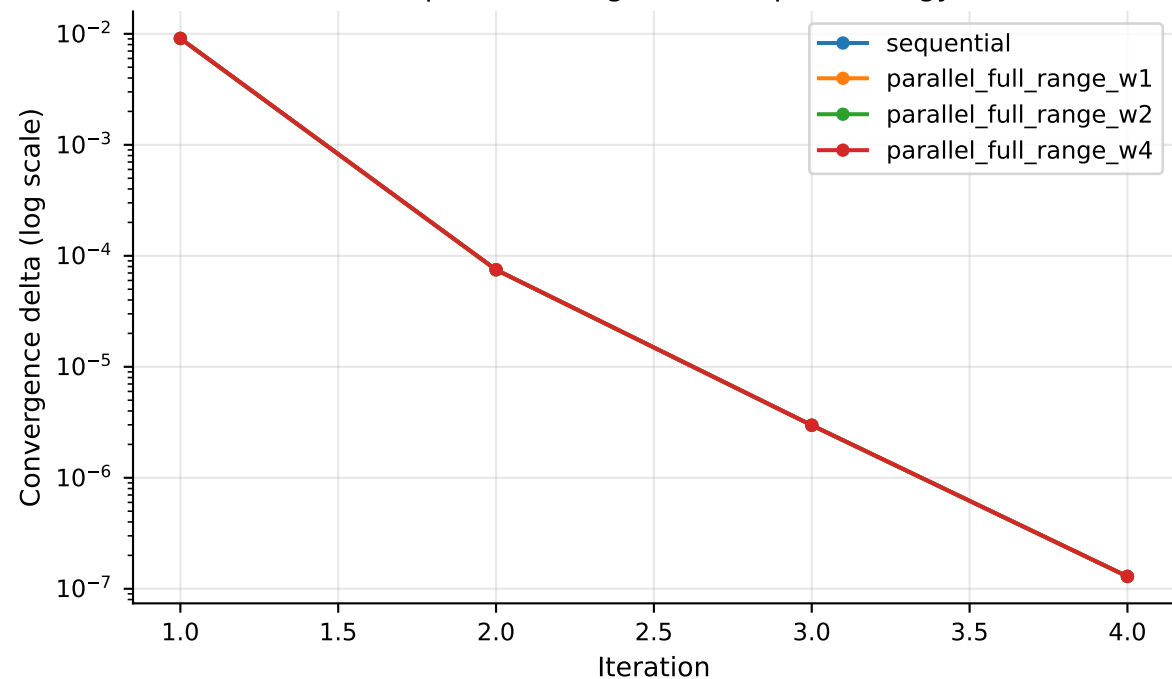
Group A - Convergence rate per strategy
